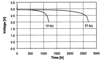
Discharge performance at 23°C
