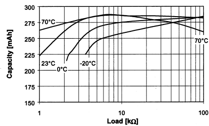
Cell capacity at various loads
